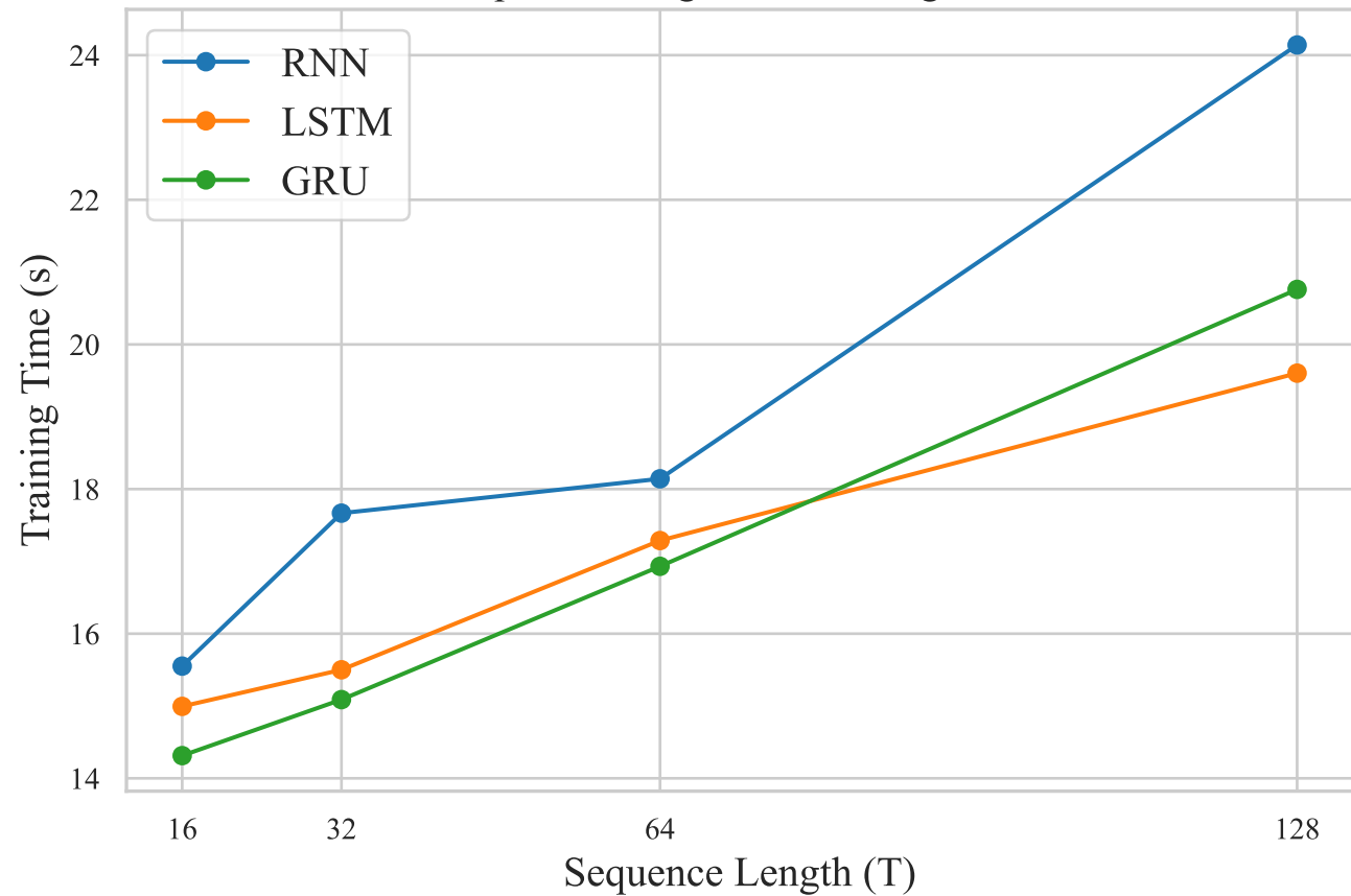
Sequence Length vs. Training Time
